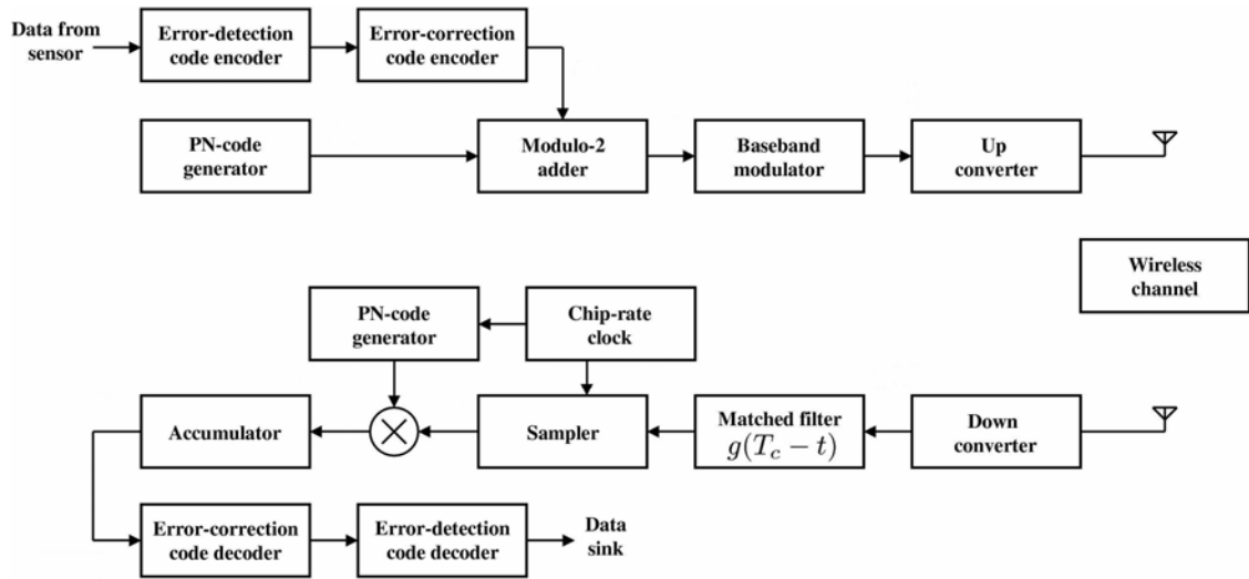
Figure 2. Schematic of Uplink Transmitter and Receiver
