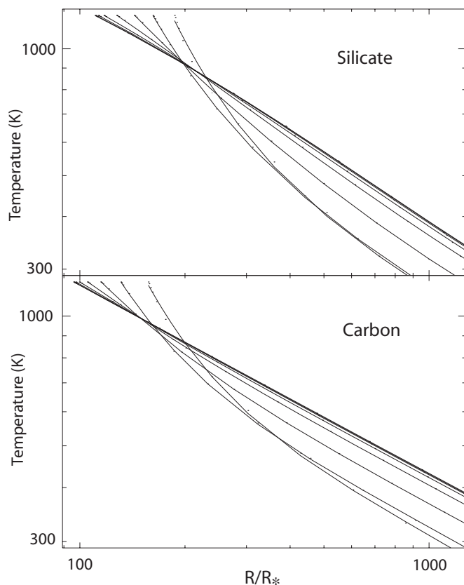
Figure 8. Temperature profiles in a spherical shell around G29-38. The top panel is for amorphous olivine, and the bottom panel is for amorphous carbon. All models are computed to an inner temperature of 1200 \text{ K} . Each profile is for a different total optical depth, with values 0.0100, 0.0268, 0.072, 0.193, 0.518, 1.39, 3.73, \text{ and } 10 . The optically thin models extend closest to the star, are the warmest at the outer edge of the plot, and are closest to a straight line ( T \propto r^{-0.5} ). The optically thick models begin further from the star and decrease in temperature much more steeply.
