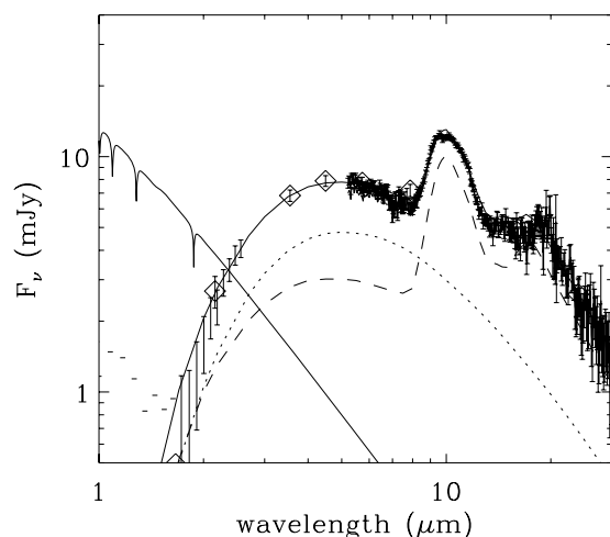
Figure 7. Spherical shell models for the dust around G29-38. Individual models for amorphous olivine and carbon are shown as dashed and dotted curves, respectively, and a linear combination is shown as the solid curve. The input white dwarf spectrum and the photosphere-subtracted infrared observations are shown for comparison. The DUSTY models have optical depth \tau(0.55 \mu\text{m}) = 0.018 and 0.011 in silicates and carbon, respectively.
