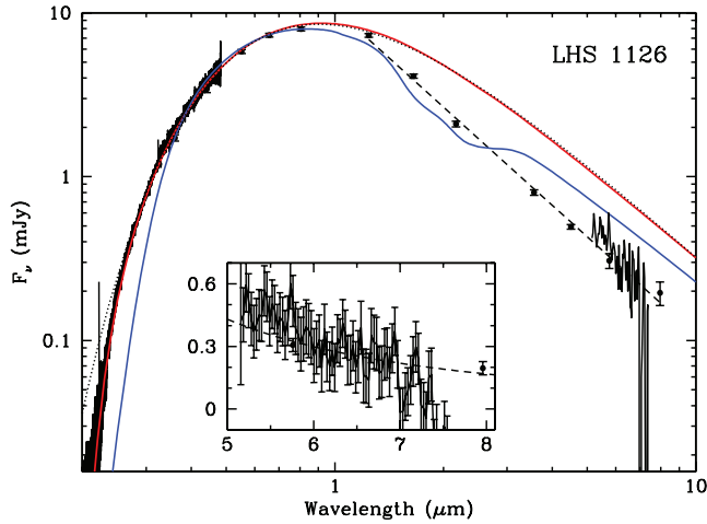
FIG. 4.—SED of LHS 1126, along with a 5400 K pure He atmosphere model (dotted line). Red and blue solid lines show the model atmospheres using the best-fit parameters from Wolff et al. [2002; T_{\text{eff}} = 5400 K, \log g = 7.9 , and \log(\text{He}/\text{H}) = 5.51 ] and Bergeron et al. [1997; T_{\text{eff}} = 5400 K, \log g = 7.9 , and \log(\text{He}/\text{H}) = 1.86 ], respectively. The dashed line shows a least-squares fit to the infrared photometry data only. The infrared portion of the SED is best fit with a power-law index of -1.99 . The inset shows the 5\text{--}8\ \mu\text{m} spectral region in detail.
