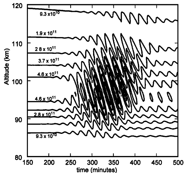
Figure 1. O density response to wave 1 as a function of altitude and time at the first horizontal grid position.
