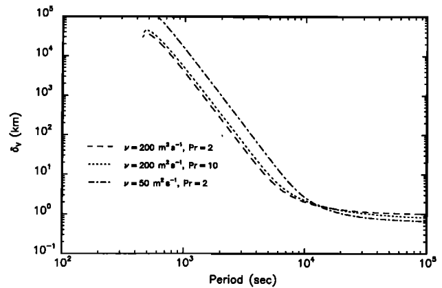
Fig. 4. The influence of different eddy diffusivity parameters on the period dependence of the vertical attenuation distance \delta_v at the peak emission height for \lambda_x = 100 km.
