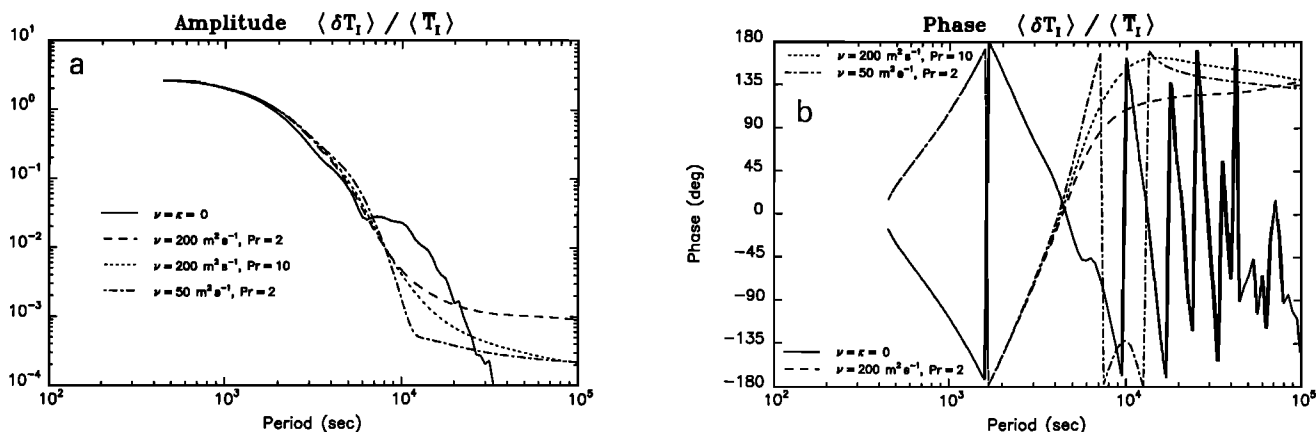
Fig. 14. Similar to Figure 12, but for the vertically integrated normalized temperature perturbation \langle \delta T_I \rangle / \langle \bar{T}_I \rangle .
