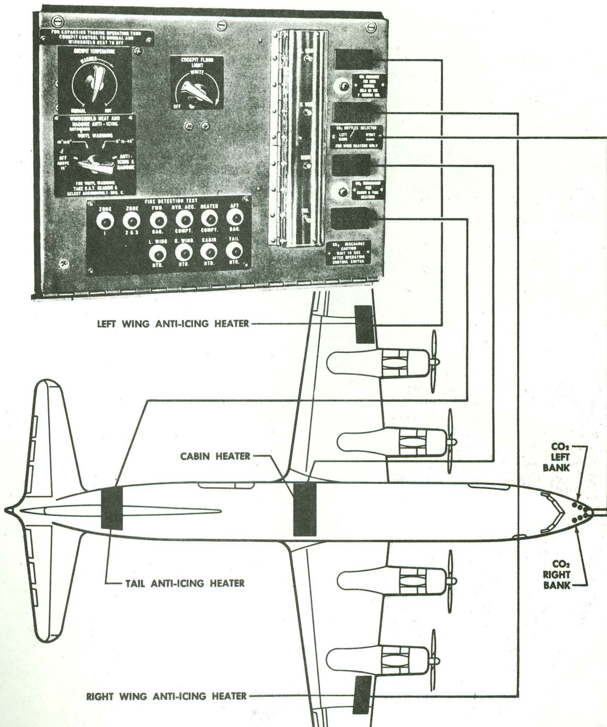
Heater Fire Protection and Control (Typical)
