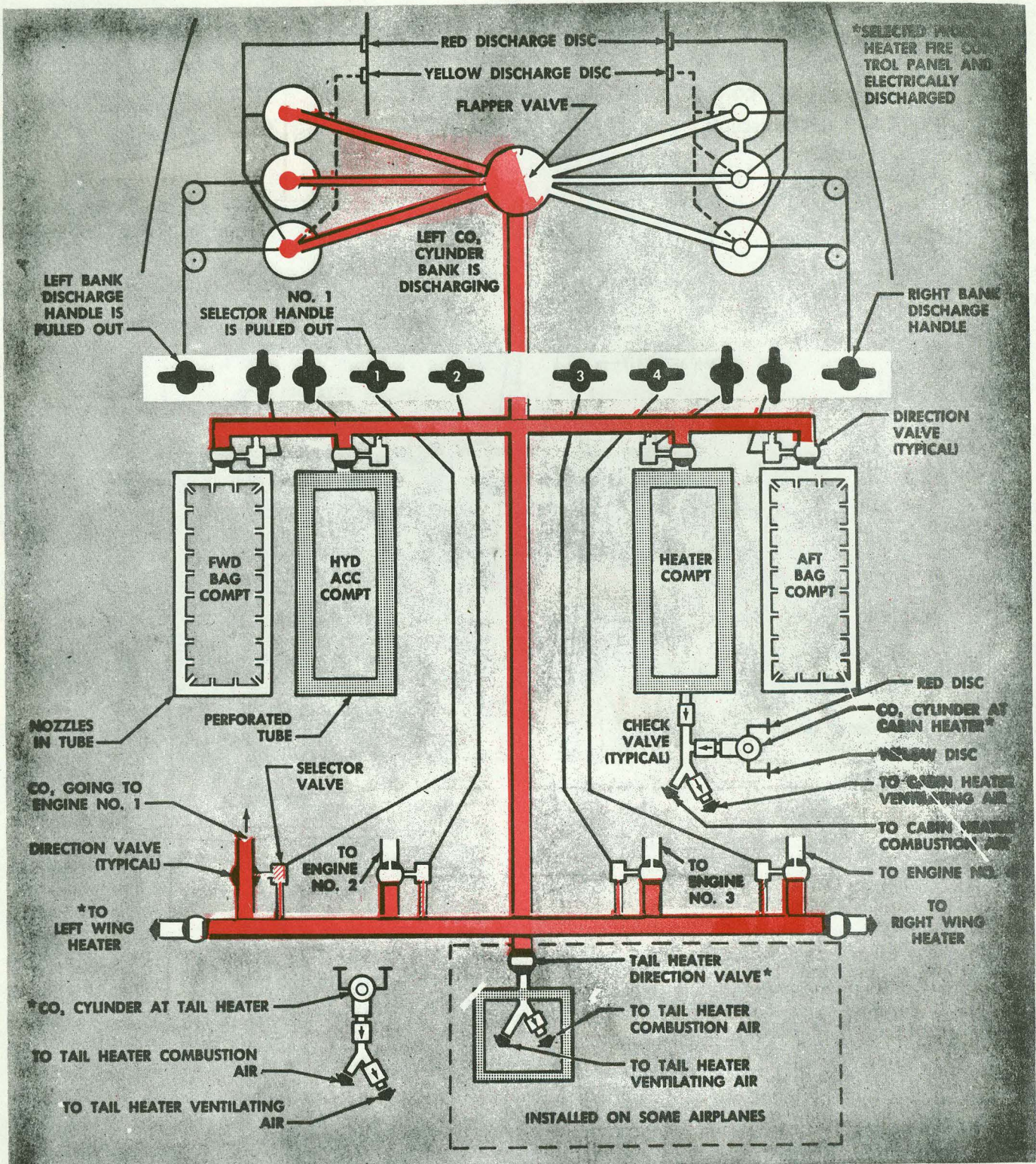
Main CO 2 System Schematic
