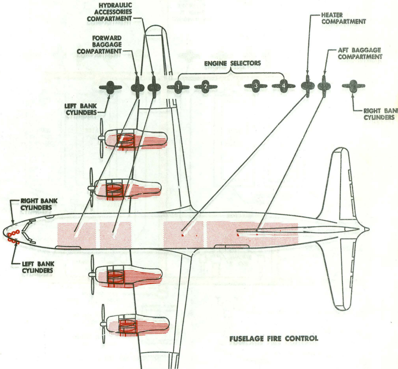
Fire Control Zones
