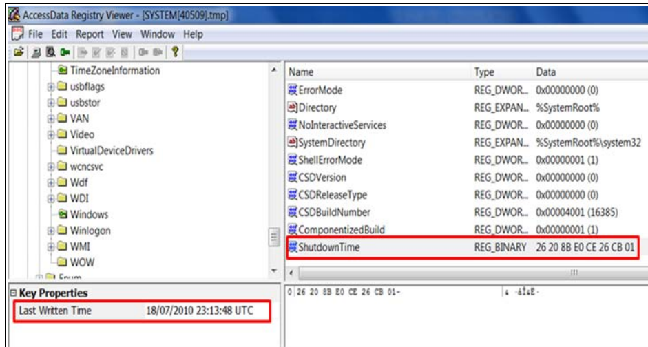
Figure 9: Shut down time value with Windows Registry
