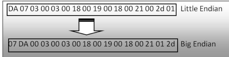
Figure 16: Convert DateCreated Registry value to big Endian format
