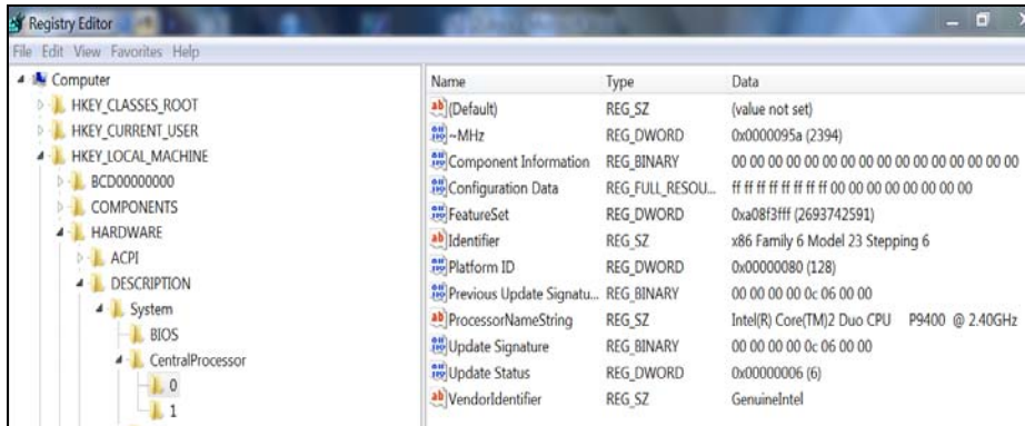
Figure 6: Central Processor description within Windows Registry
