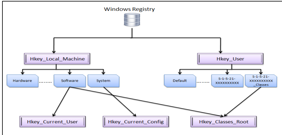
Figure 3: Relation between Windows Registry root keys
