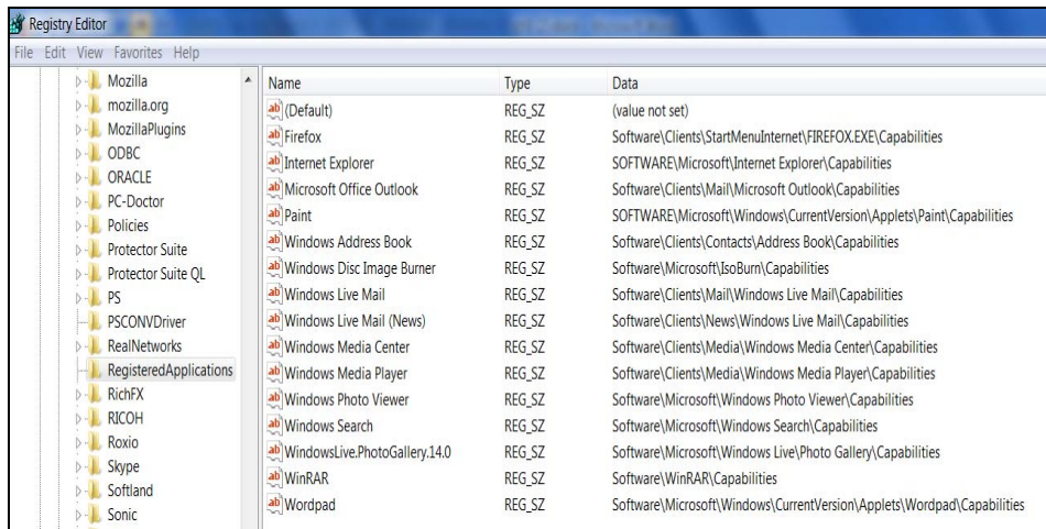
Figure 11: List of Registered application within Windows Registry
