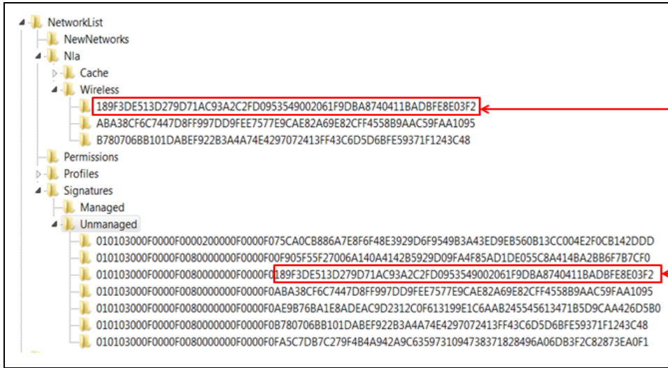
Figure 14: Matching Wireless network identifier within Windows Registry
