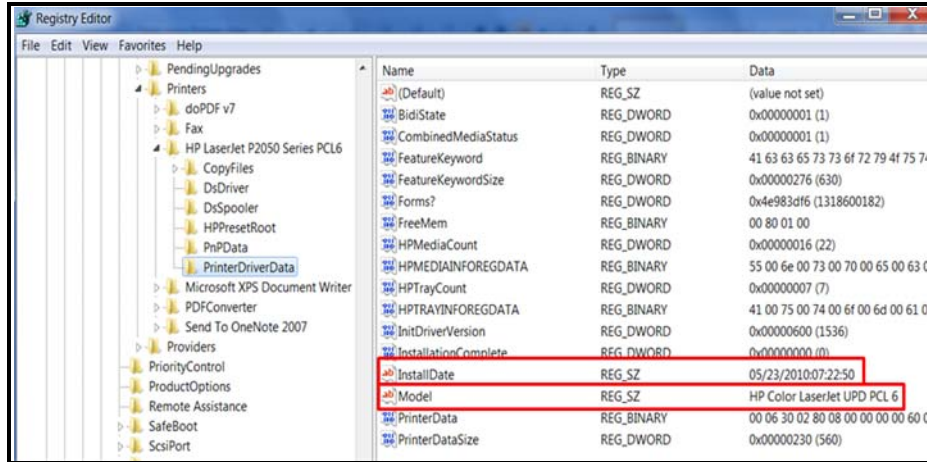
Figure 17: Valuable forensics elements of printer drive within Windows Registry
