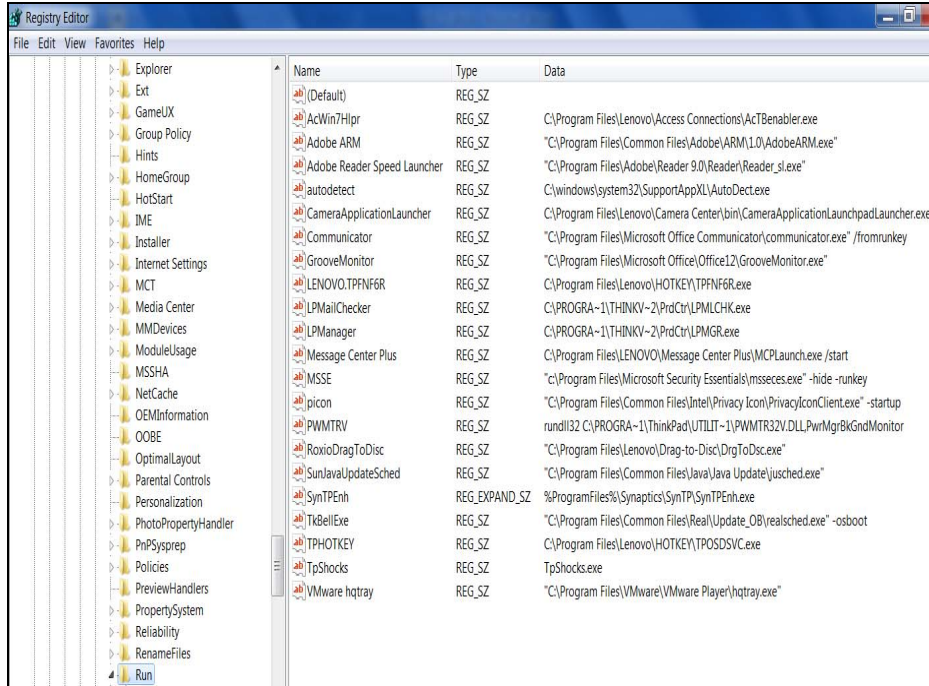
Figure 10: List of startup programs with Windows Registry
