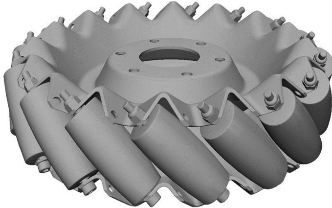
Figure 1.2 Mecanum Wheel with Rollers: [4].
