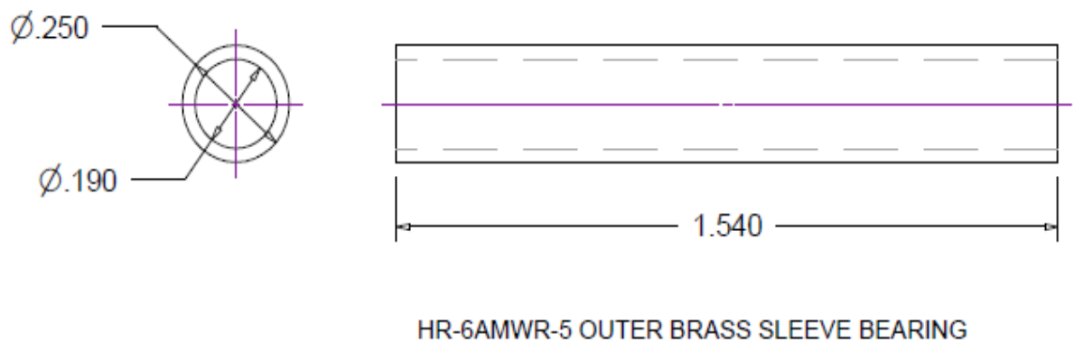
Figure 2.1 Dimensions of Brass Sleeve & Bearing: [9].
