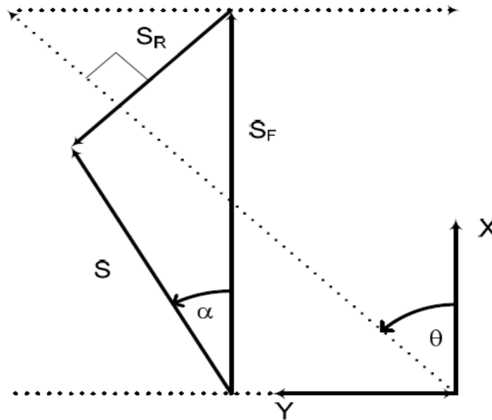
Figure 2.4 Displacement Vector: [11].
