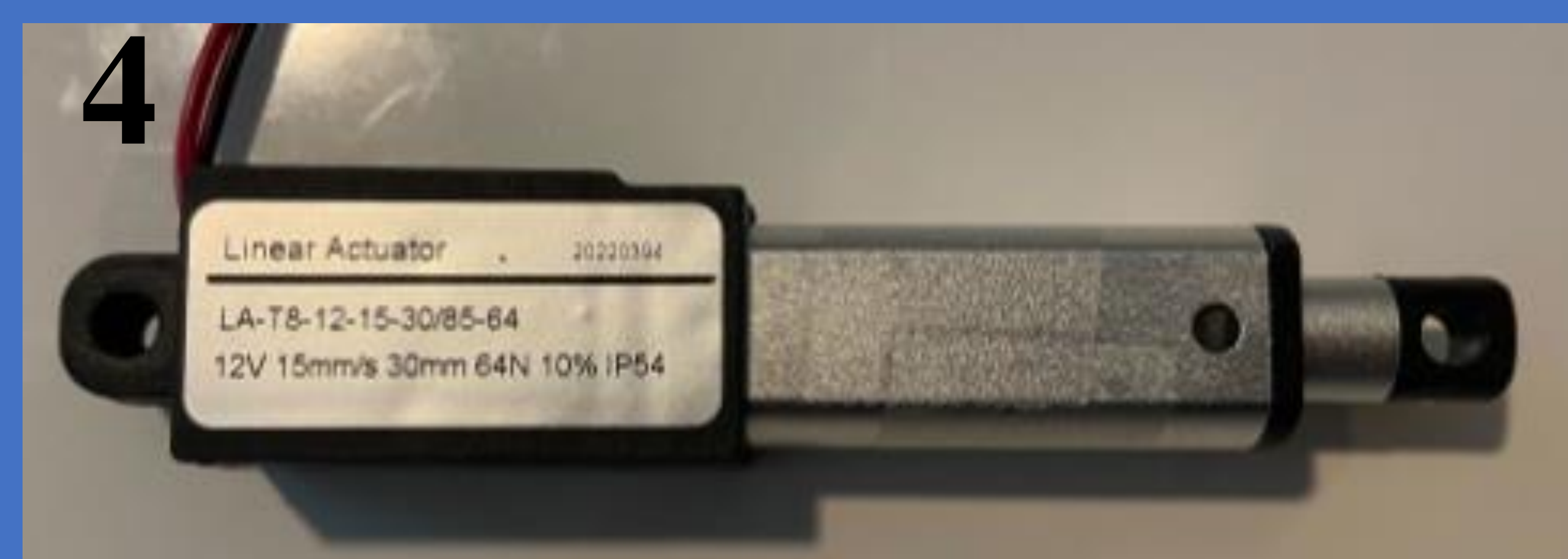
Image 4: Mini Linear Actuator used to move the plate that holds the magnet in the M.A.S. These actuators can be programmed to actuate at specific frequencies.
