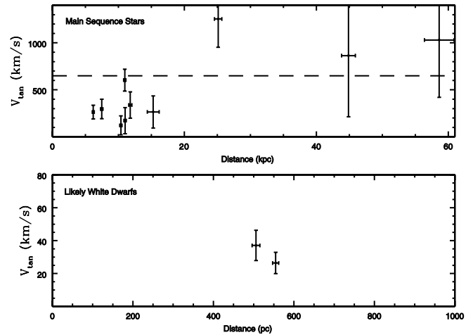
FIG. 7.—Tangential velocities and distances for main-sequence stars ( top panel ) and likely white dwarfs ( bottom panel ) brighter than 27th magnitude. The dashed line marks the upper bound for the escape velocity from the Milky Way ( 650 \text{ km s}^{-1} ; Leonard & Tremaine 1990; Meillon et al. 1997). All of the main-sequence stars have halo properties, whereas the probable white dwarfs have disk properties.
