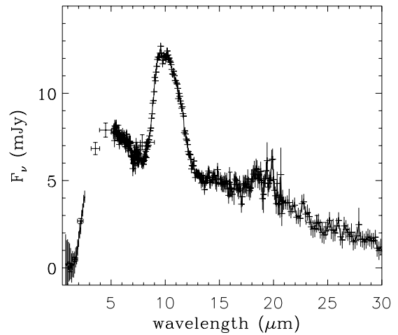
Figure 3. Combined spectra and photometry (using 2MASS, IRTF, IRAC, MIPS, and IRS) of G29-38 with stellar photosphere removed.
