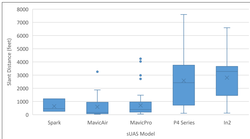
Figure 5. Box & Whisker plot of detected sUAS Max Slant Flight Distances by platform type plotted in feet.
