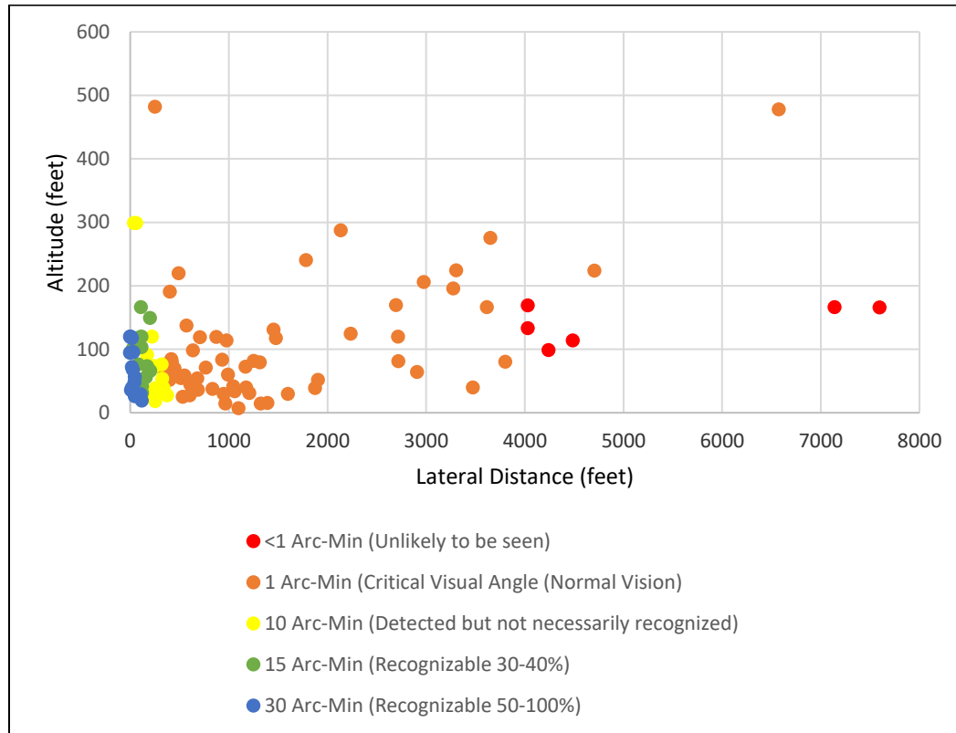
Figure 8. Model of Greening (1976) visibility based on UAS distance and altitude of aerial vehicle relative to operator position, plotted in feet.
