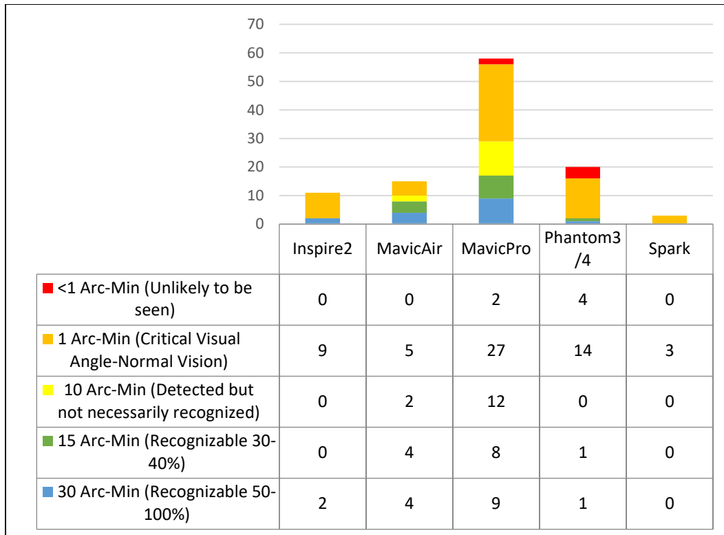
Figure 6. Detected sUAS model visibility based on Greening (1976) visibility modeling.
