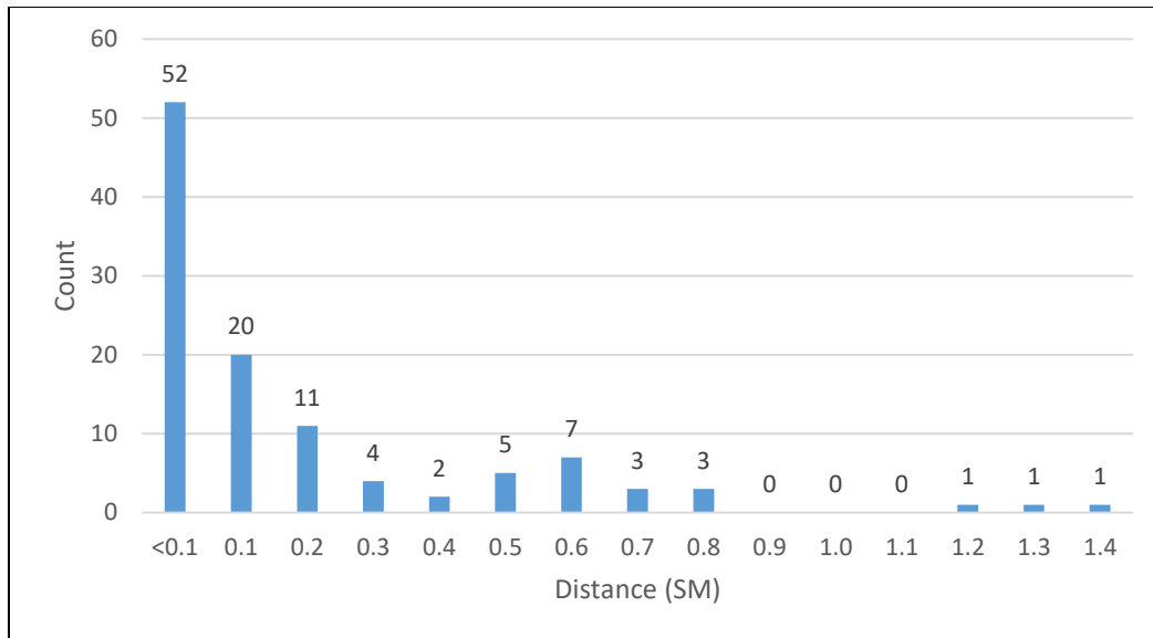
Figure 4. Histogram of detected sUAS max slant range in 1/10 SM bins.
