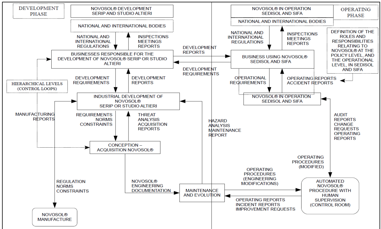
Fig. 1 An analysis of novosol® using the stpa technique, the structure takes into account the development and operation of novosol®, and shows the interactions between hierarchical levels [5, 8].
