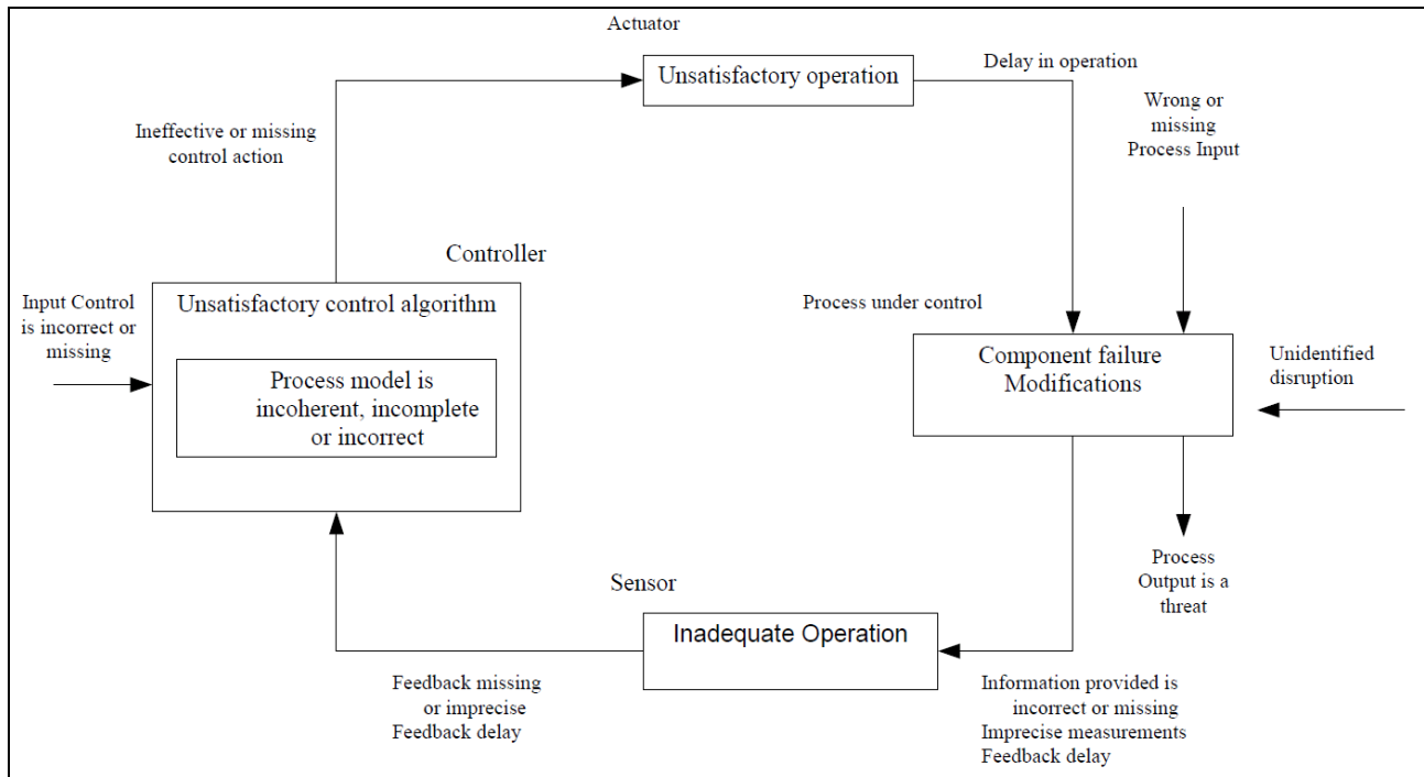
Fig. 2 Defects in the control loop, finding weaknesses in a control loop enables inadequate control actions to be identified.
