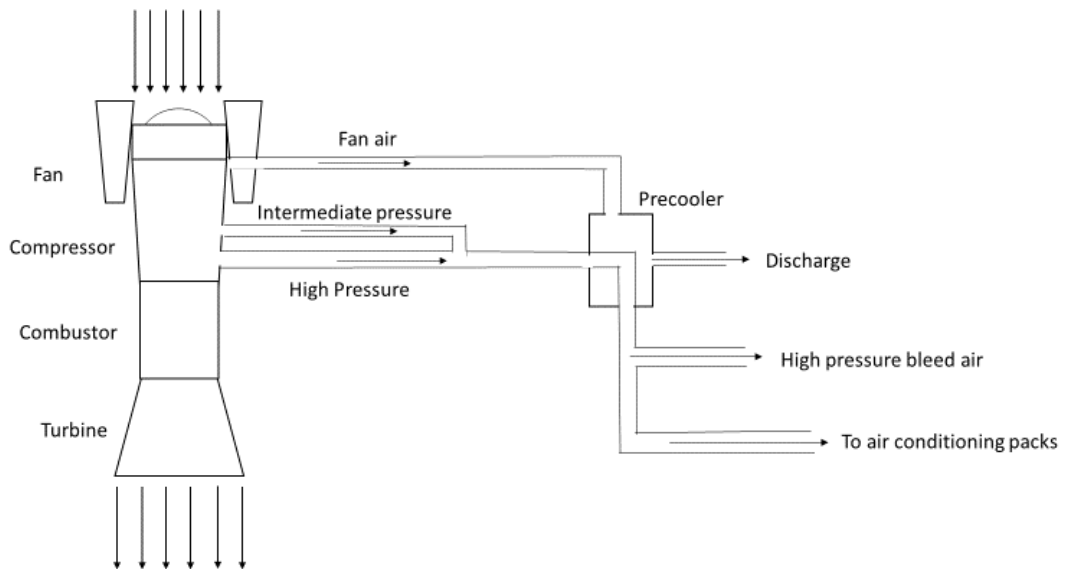
Typical Basic Aircraft Bleed Air System"
