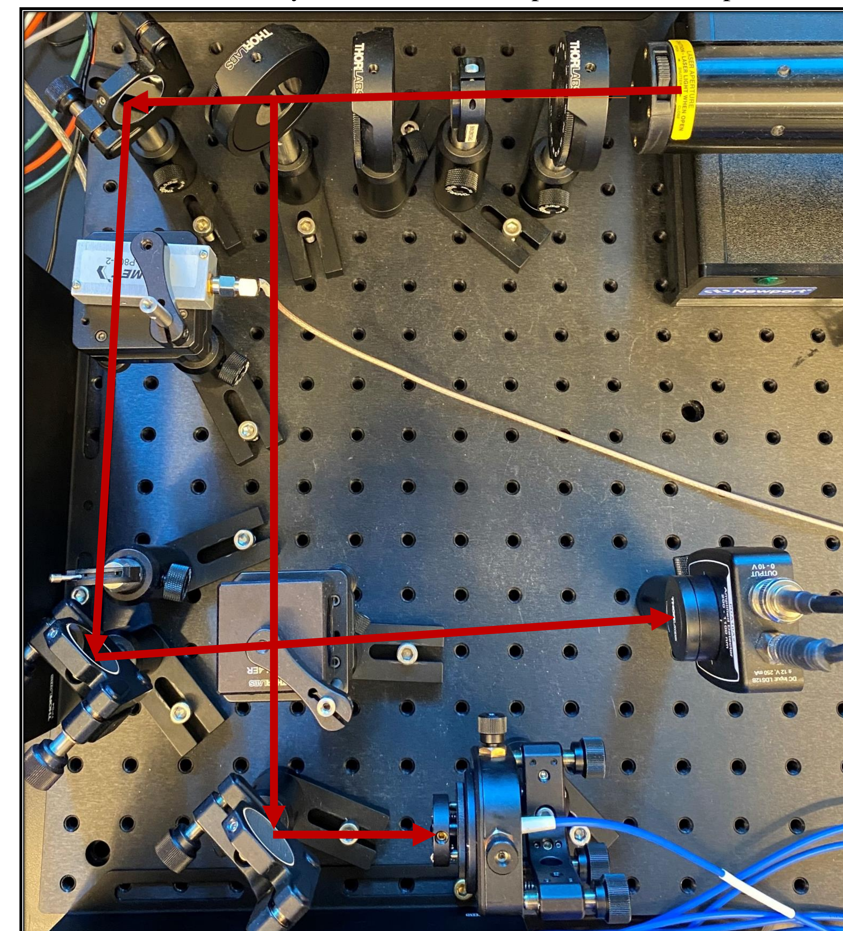
Heterodyne Interferometer Optics Bench Setup
