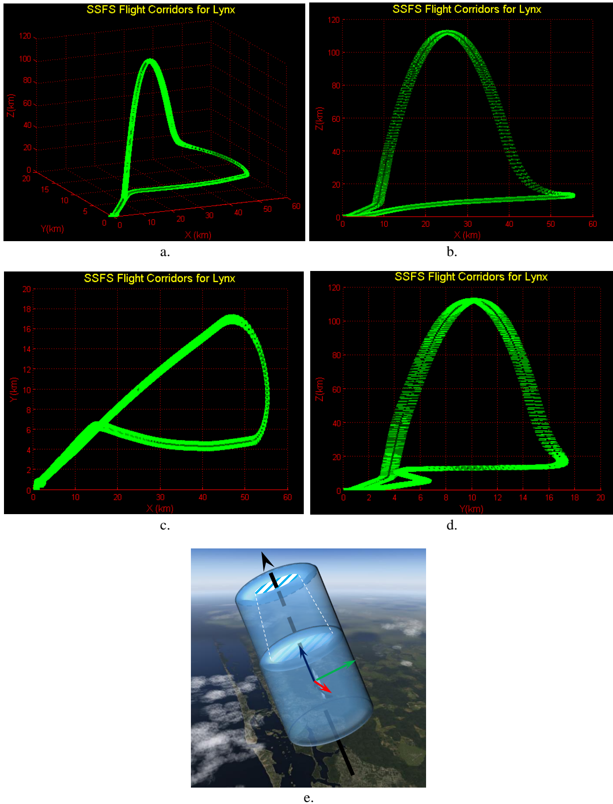
Figure 1. Space Transition (Flight) Corridors using the Lynx platform: (a) 3D trajectory of XCOR Lynx, (b) xz -projection of trajectory, (c) xy -projection of trajectory, (d) yz -projection of trajectory, (e) Sketch of the FTCs showing the safety limits for a nominal mission.
