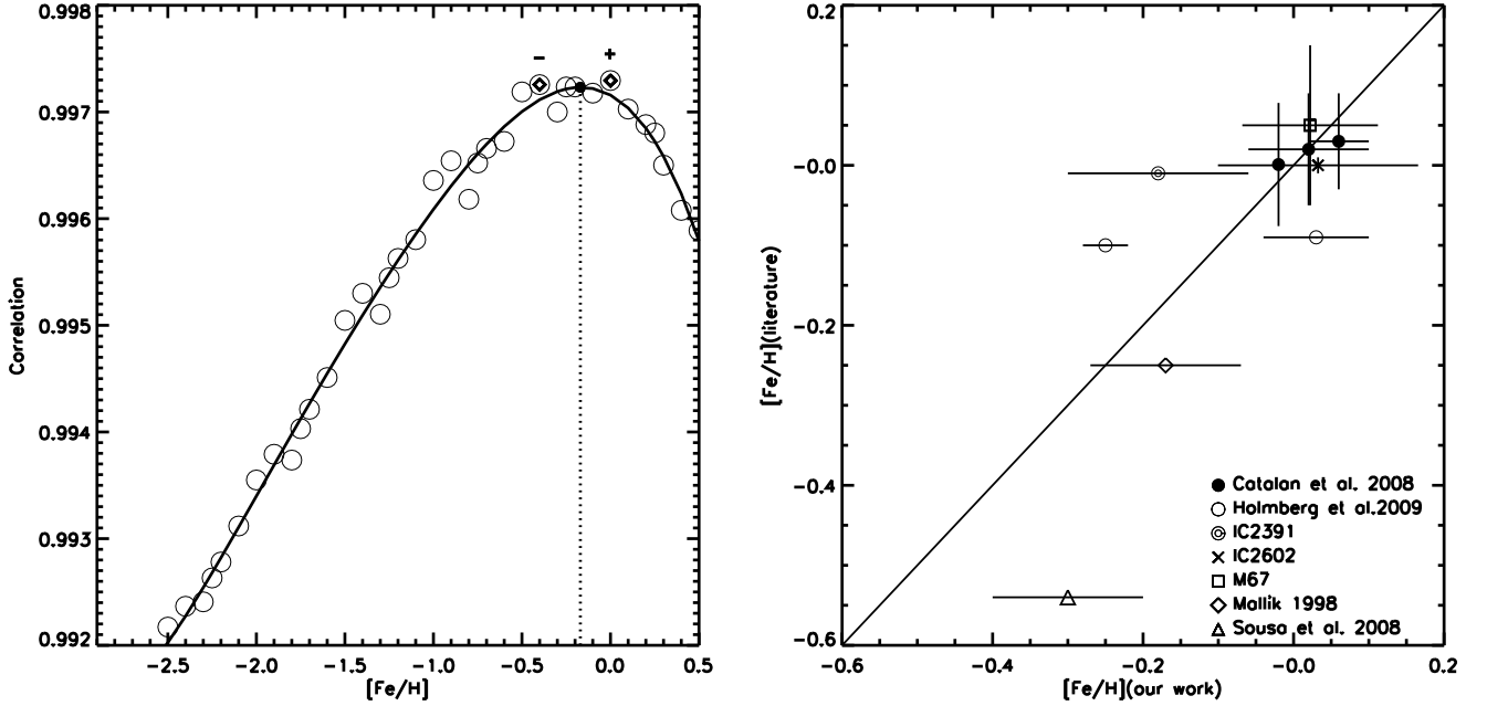
Fig. 3.— Left: An example of how [\text{Fe}/\text{H}] estimates were made with the maximum correlation method. The filled circle is the maximum of fitted polynomial. The [\text{Fe}/\text{H}] correlated to this maximum is regarded as our final result. + and - signs indicate our estimate of uncertainty as discussed in the text. Right: The comparison between our [\text{Fe}/\text{H}] results and those in the literature. Filled circles represent stars in Catalán et al. 2008a. Single open circles represent stars in Holmberg, Nordström & Andersen (2009). Double open circles, X signs and squares represent the clusters IC2391, IC2602 and M67, respectively. We adopted the average [\text{Fe}/\text{H}] of member stars as the final cluster [\text{Fe}/\text{H}] . The [\text{Fe}/\text{H}] of IC2391 and IC2602 are from D’Orazi & Randich (2009), while that of M67 is from Pancino et al. 2010. Diamonds and triangles represent stars in Mallik (1998) and Sousa et al. (2008), respectively. Note that many of these sources did not give uncertainties, hence no vertical error bar could be plotted.
