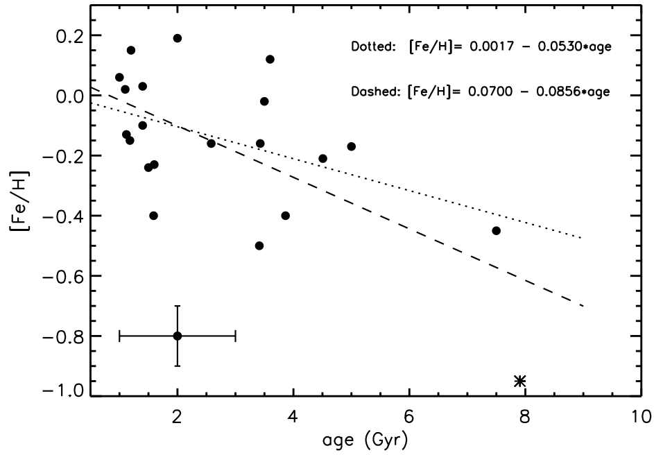
Fig. 4.— Our [Fe/H] vs. age relation for 21 MS stars. Typical uncertainties in age and [Fe/H] are displayed at the lower left of this figure. Filled circles represent disk stars. Only one star indicated by an asterisk (LHS300A) is a likely halo star. The dotted line is a least-squares fit for only disk stars, while the dashed line includes all stars.
