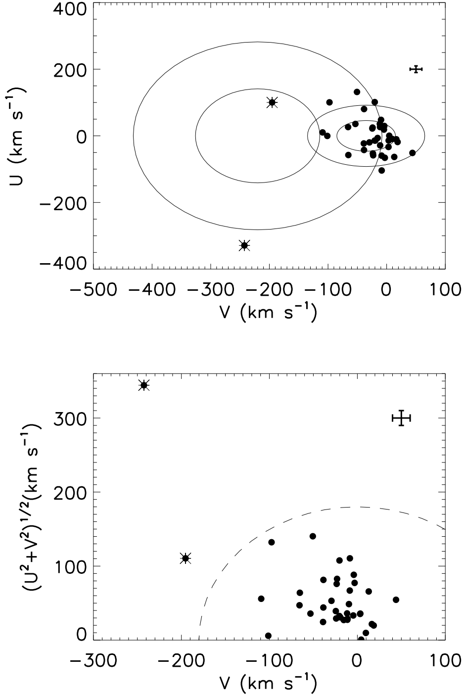
Fig. 5.— Top: UV-velocity distribution of our sample with measured v_r ( \text{km s}^{-1} ). The ellipsoids indicate the 1\sigma (inner) and 2\sigma (outer) contours for Galactic thick-disk and stellar halo populations, respectively. Typical error bars are given in both panels. Bottom: Toomre diagram of our stars. Dashed line is V_{total} = 180 \text{ km s}^{-1} .
