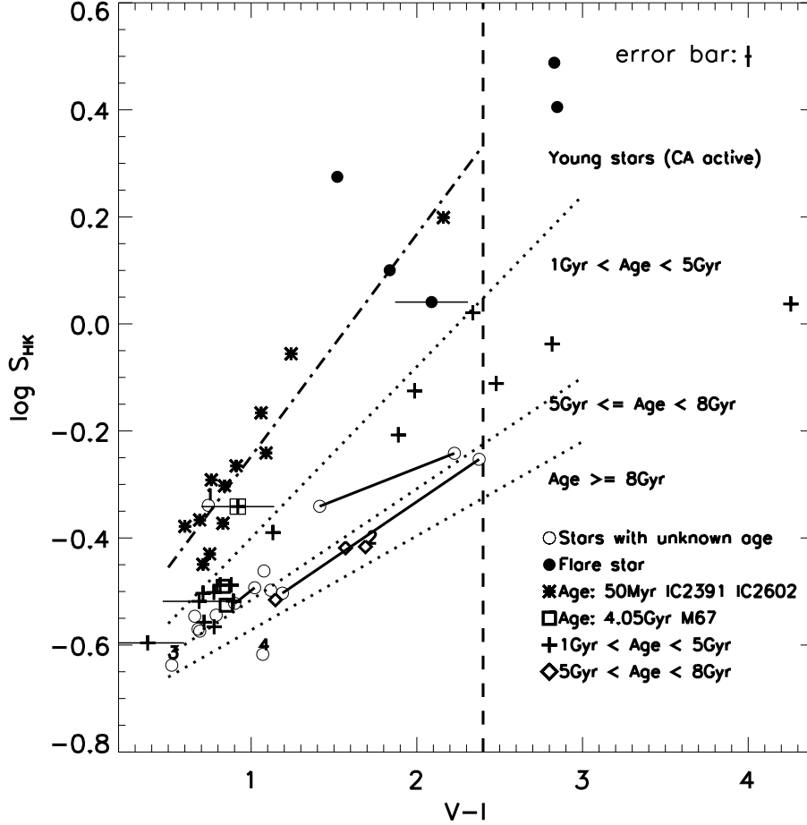
Fig. 2.— The relation among \log(S_{\text{HK}}) , V-I and age. Open circles represent CPMB stars with unknown age. Filled circles are flare stars. Stars in cluster IC2602 + IC2391 and M67 are shown as asterisks and squares respectively. Plus signs and diamonds represent stars with different ages: 1\text{Gyr} < \text{age} < 5\text{Gyr} and 5\text{Gyr} < \text{age} < 8\text{Gyr} , respectively. Four domains are divided by dotted lines. The dash-dot line is the least-squares fit of young clusters IC2602+IC2391. The vertical dashed line is V-I = 2.4 . To the right of this, CA is not expected to depend on age. Solid lines connect the MS components in CD-31 7352/LP902-30, LP684-1/2 and LP387-1/2. The star indicated as number 1 is G163-B9A. Numbers 2-3 denote halo star candidates (LHS300A and CD-31 1454). Number 4 is the star with the weakest activity in our sample (G114-B8B). The typical error bar for our measurement is in the upper right corner. Separate V-I uncertainties are given for 4 stars whose V-I were estimated by the relation in Fig.1. A square with a plus sign is an outlier (G95-B5A) that seems overactive for its age domain. This star is perhaps a close binary and it warrants follow-up observations to determine the cause of its high CA.
