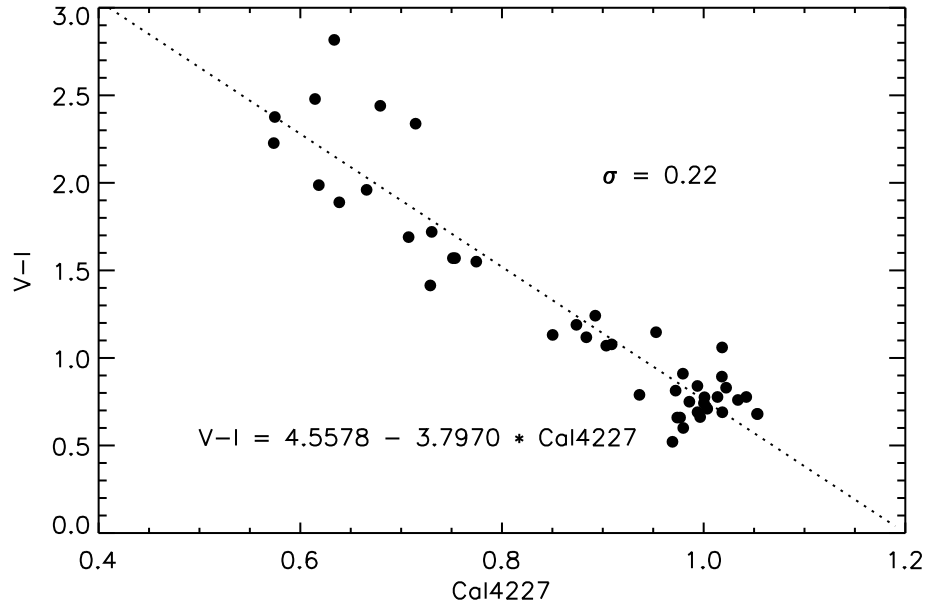
Fig. 1.— The relation between V-I and flux ratio of CaI4227. The dotted line is a least-squares fit. We used this relation to estimate V-I color for a few stars whose photometric data was unavailable. See text for details.
