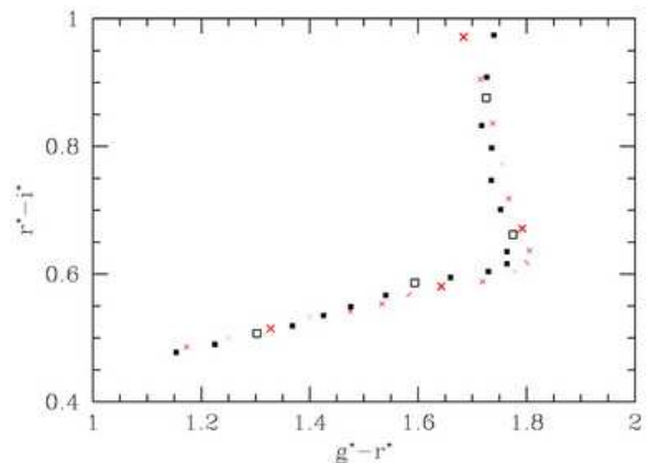
Figure 4: Black squares: colors of elliptical galaxies as a function of redshift; Red crosses: Passively evolving stellar population model (Eisenstein et al. 2001).
