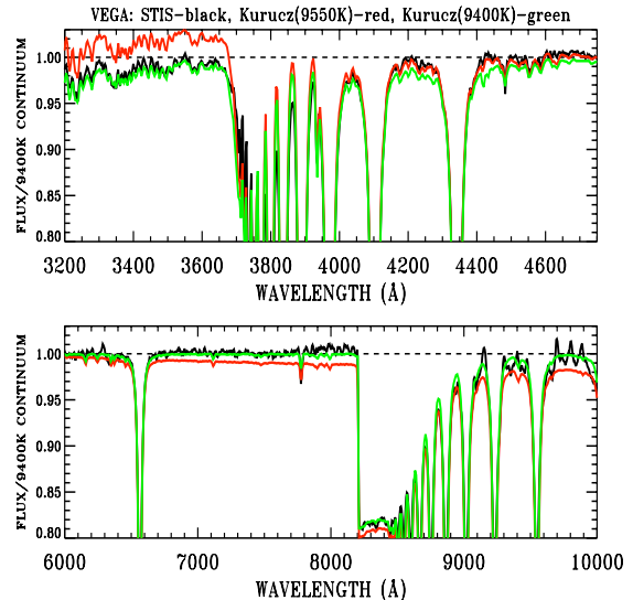
Figure 6: Uncertainties in the absolute flux for Vega: HST /STIS observations (black line: Bohlin 2007; Bohlin & Gilliland 2004), the Kurucz stellar model with T_{\text{eff}}=9400\text{ K} (green), and the Kurucz stellar model at 9550\text{ K} (red) are compared. The observations exhibit better agreement with the cooler model at the longer and shorter wavelengths. The hotter model agrees better with the measured flux by \sim 1\% at 4200–4700 Å.
