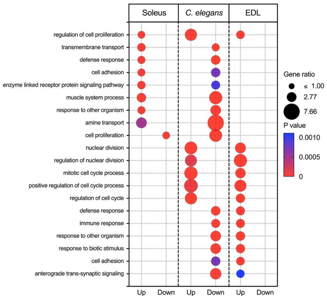
Figure 3. Shared upregulated and downregulated biological processes in C. elegans compared with soleus and the EDL in response to spaceflight. The resulting gene ratio and P values from Webgestalt analysis of DEGs are shown.
