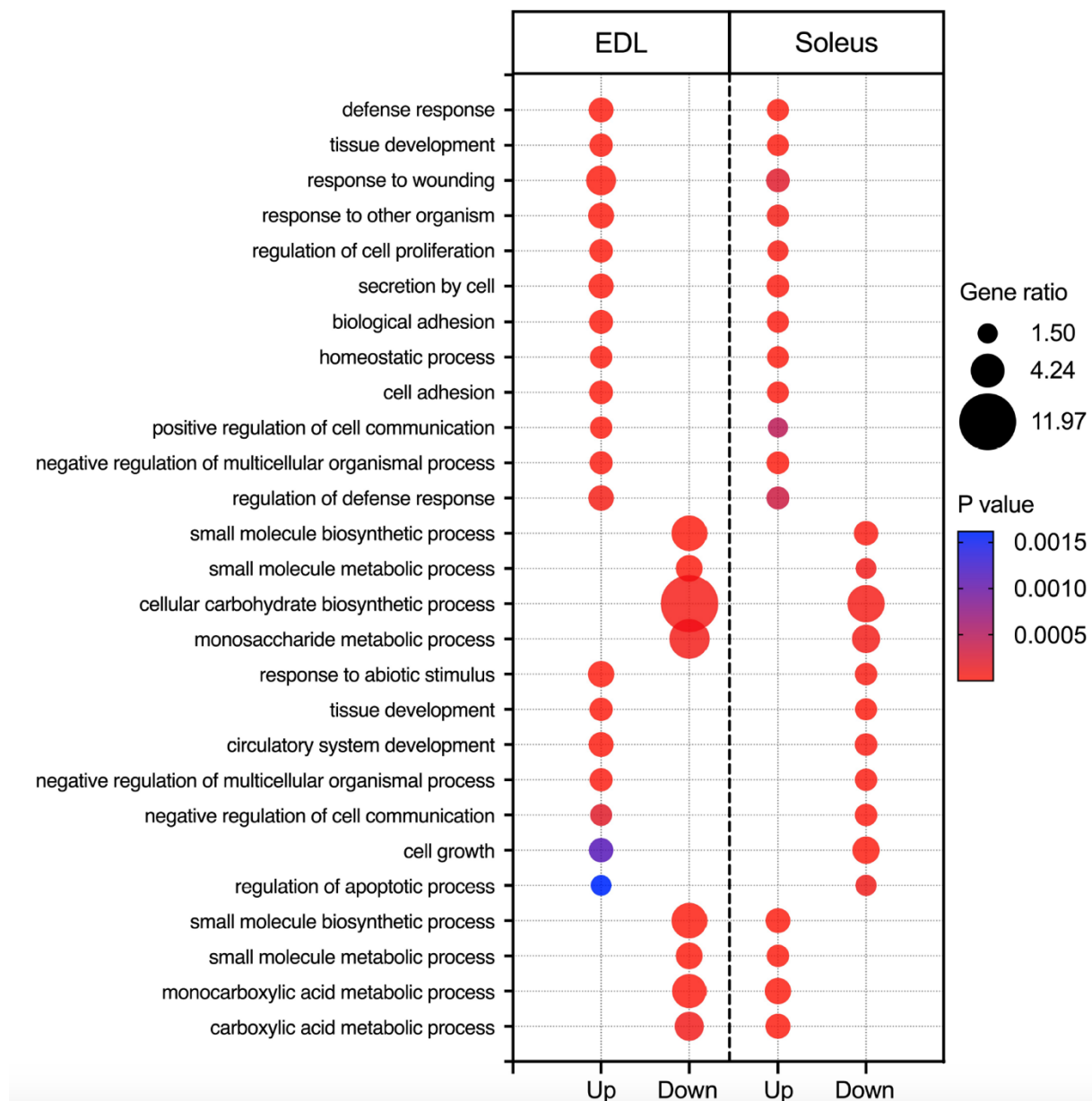
Figure 2. Shared upregulated and downregulated biological processes in soleus and EDL in response to spaceflight. The resulting gene ratio and p values from Webgestalt analysis of DEGs are shown.
