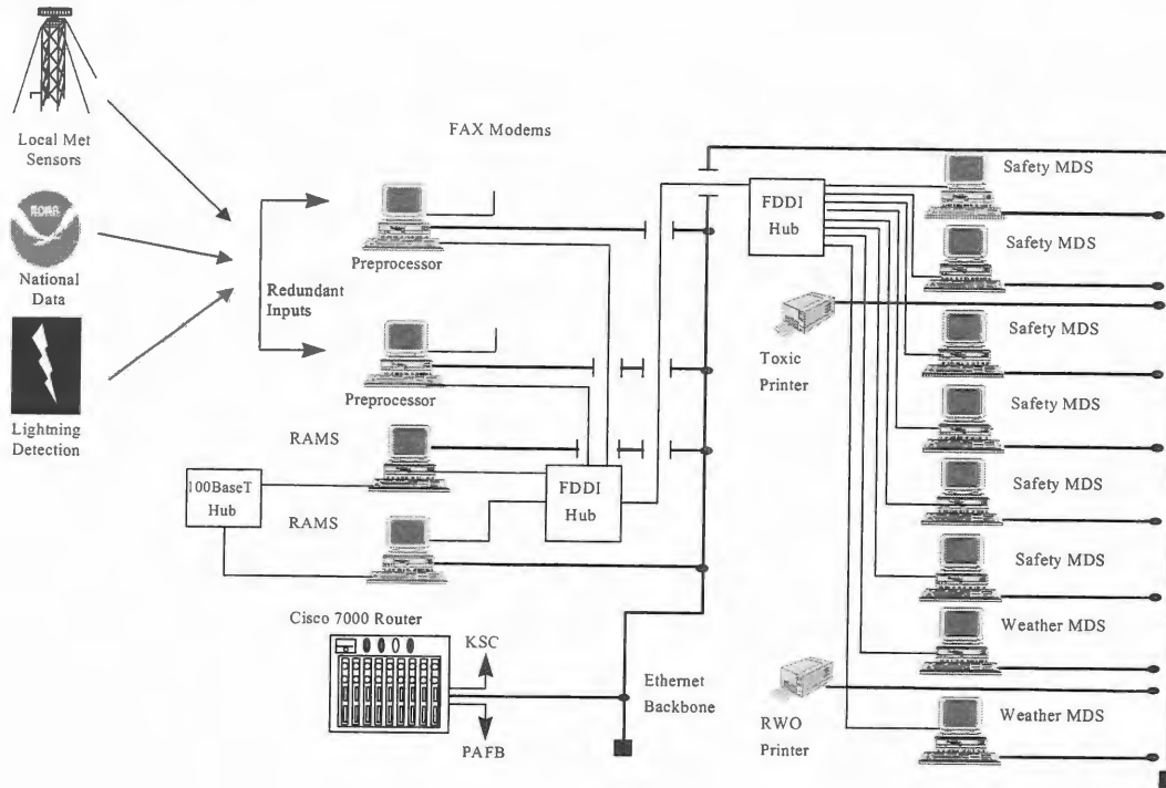
Figure 1. MARSS System
