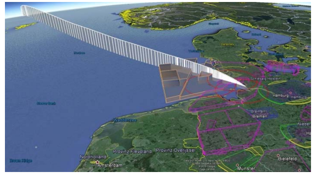
Figure 2: SpaceLiner descent trajectory for destination in northern Germany; showing also danger areas, restricted areas and temporary restricted areas within German airspace 1
